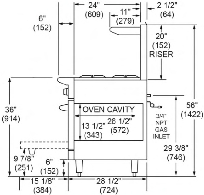
Side Super Saver Oven Base
