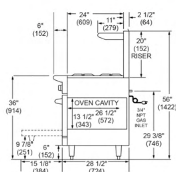
Side Space Saver Oven Base
