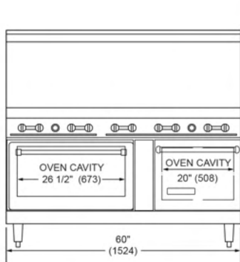
Front Oven Base
